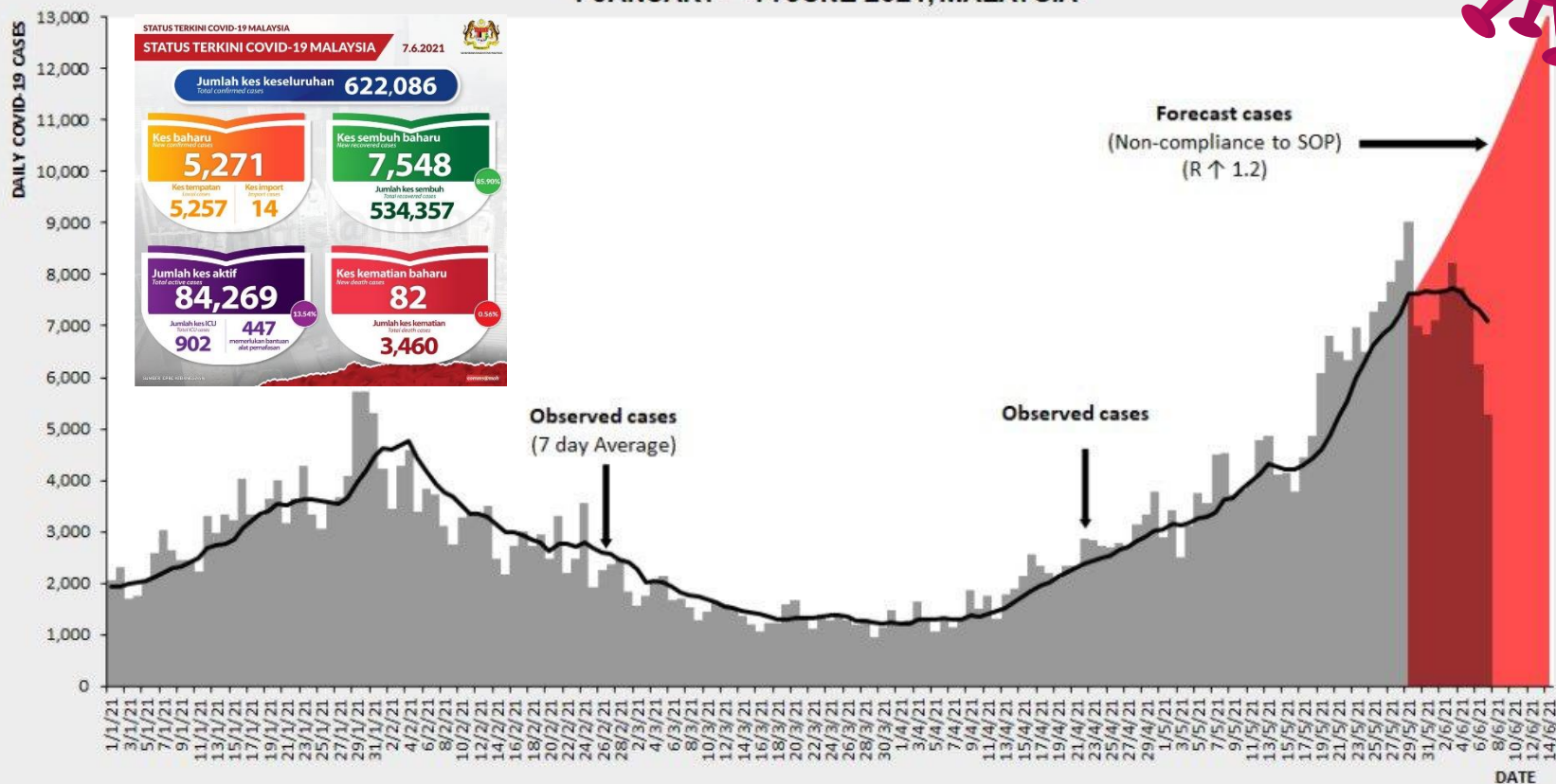
SEIR MODEL OF COVID-19 DAILY OBSERVED AND FORECAST CASES 1 JANUARY – 14 JUNE 2021, MALAYSIA
